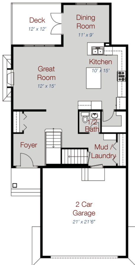
MAIN FLOOR PLAN 946 sq ft
