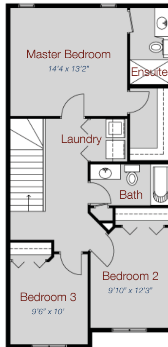
UPPER FLOOR PLAN 671 sq ft
